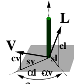
Figure 3: A single needle.
