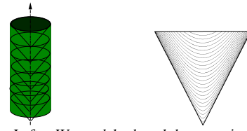
Figure 6: Left : We model a bough by a semi-opaque volumetric cylinder, which opacity is anisotropic in order to reproduce the variation of the number or intersection between a ray and the sub cones.
